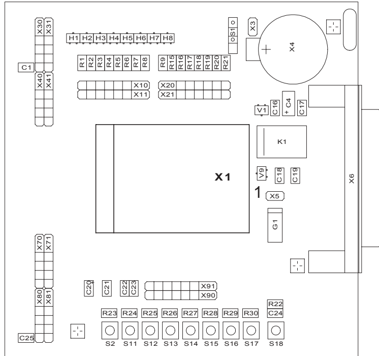
Figure 2 : XE8000EV103 implantation map
